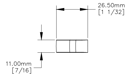
RIGHT VIEW
