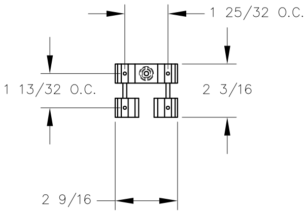
TOP VIEW OF TOP PLATE: NOT TO SCALE
