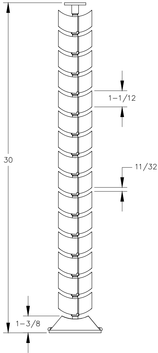
FRONT VIEW
