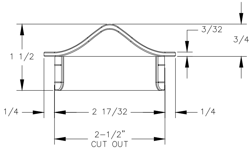
FRONT VIEW
