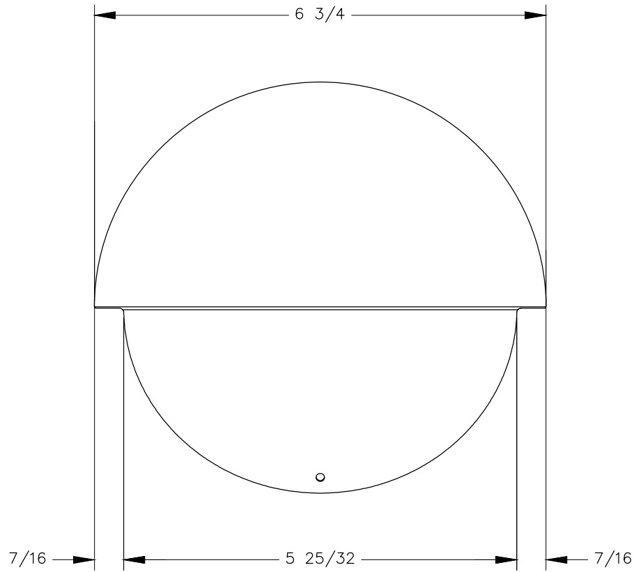
TOP VIEW
