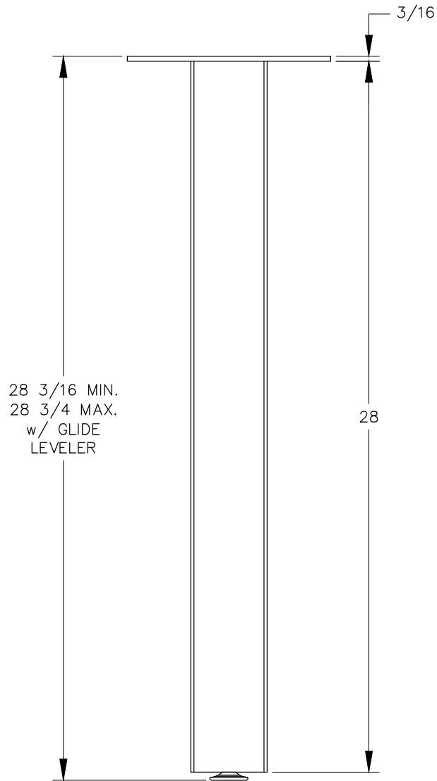
FRONT VIEW
