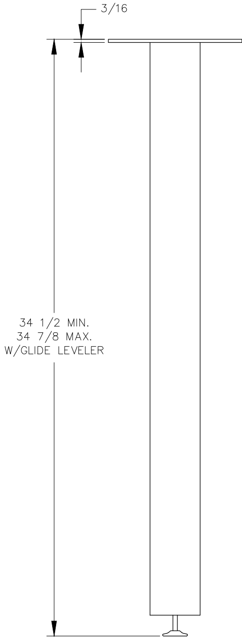
FRONT VIEW
