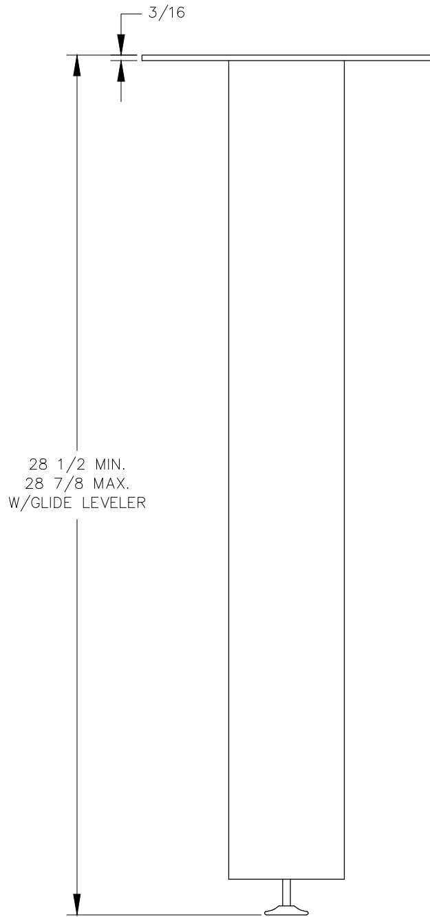
FRONT VIEW
