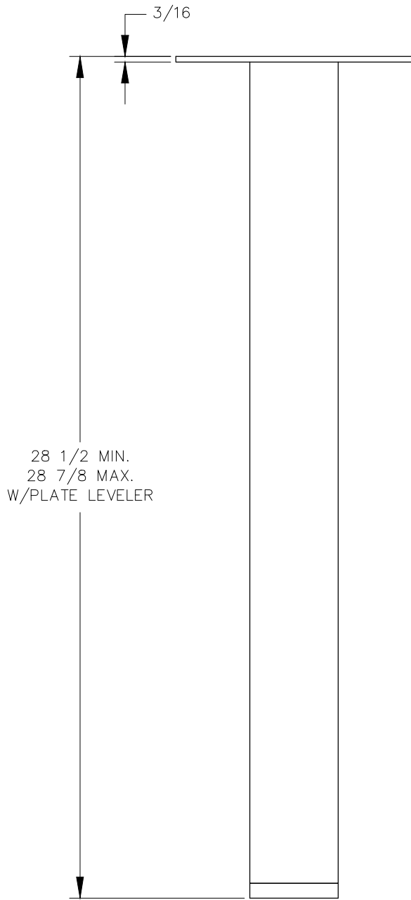
FRONT VIEW
