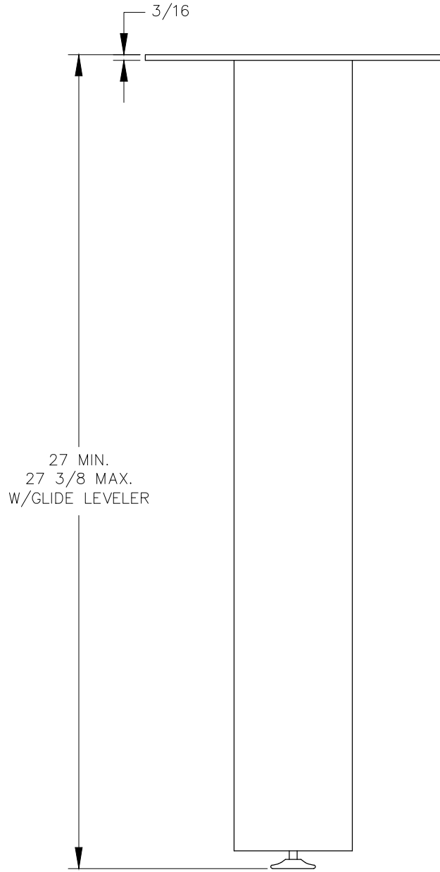
FRONT VIEW
