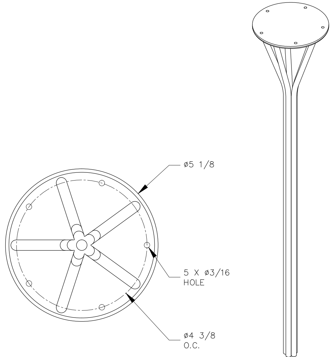
BOTTOM VIEW
