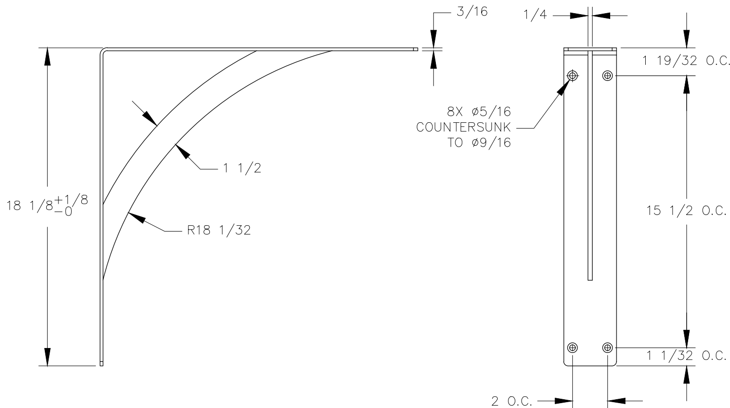
FRONT VIEW
