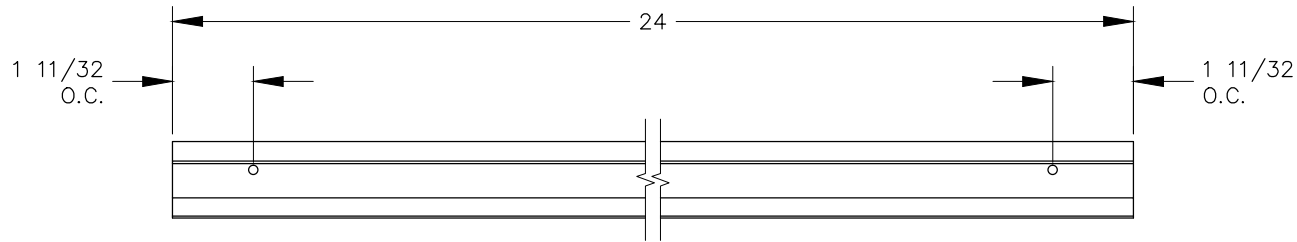
TOP VIEW
