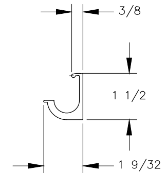
RIGHT VIEW
