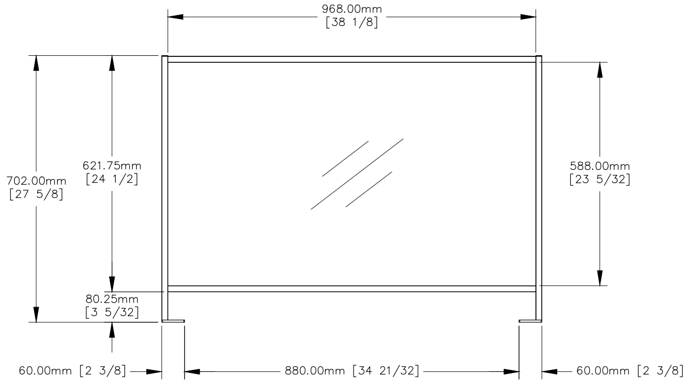
FRONT VIEW
