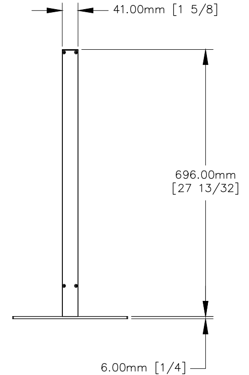
RIGHT VIEW
