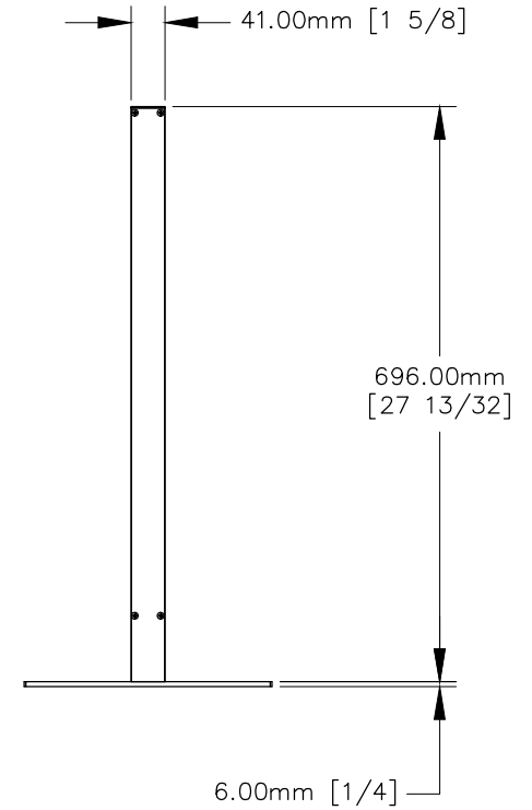
RIGHT VIEW
