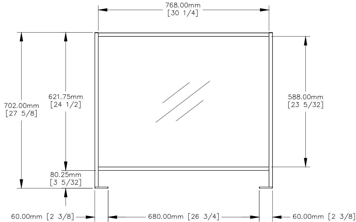
FRONT VIEW
