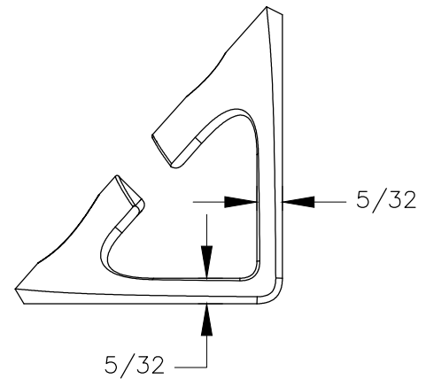
RIGHT VIEW
