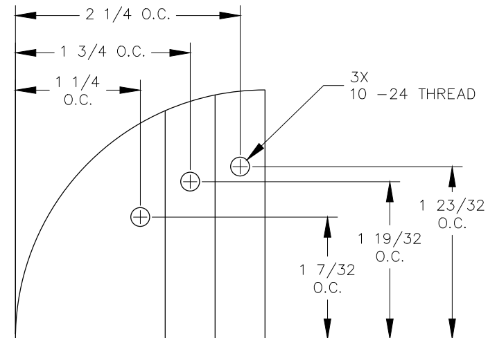
REAR VIEW
