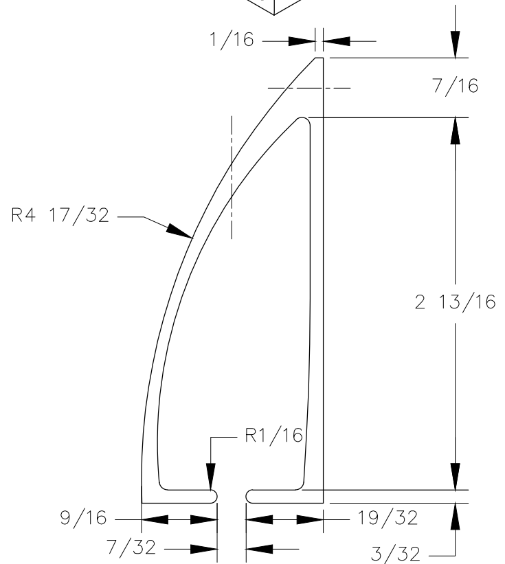
RIGHT VIEW
