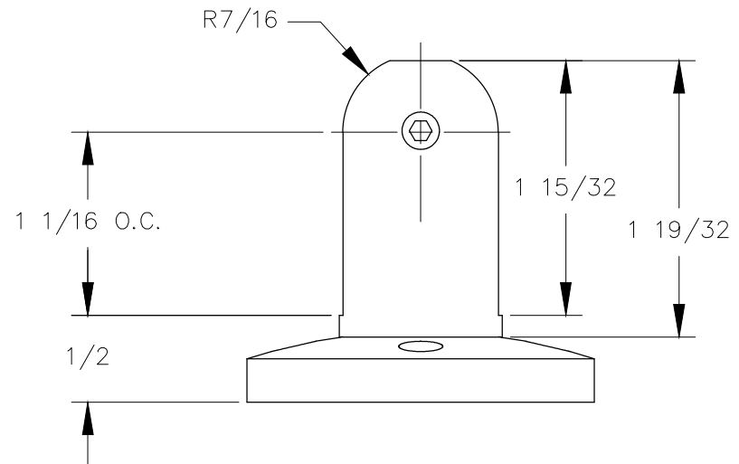
RIGHT VIEW
