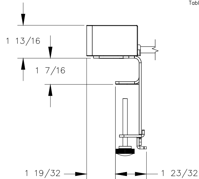
RIGHT VIEW
