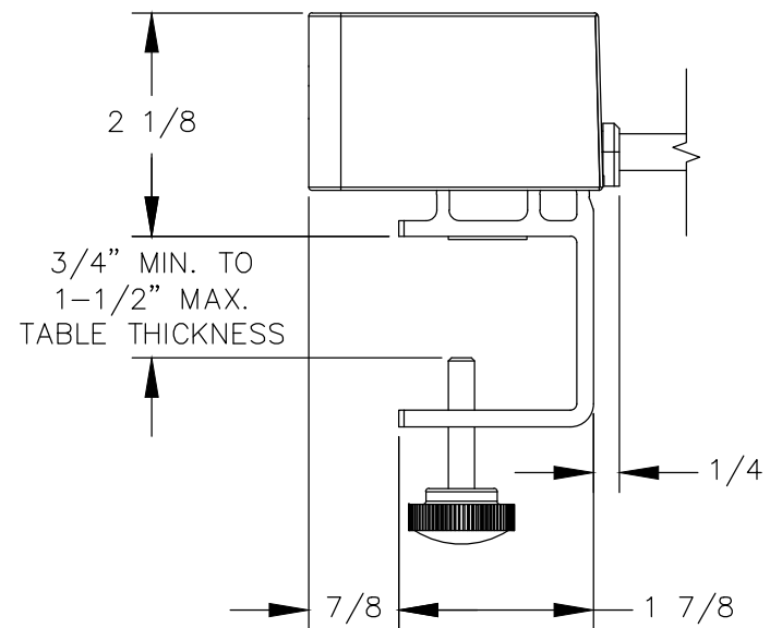
RIGHT VIEW
