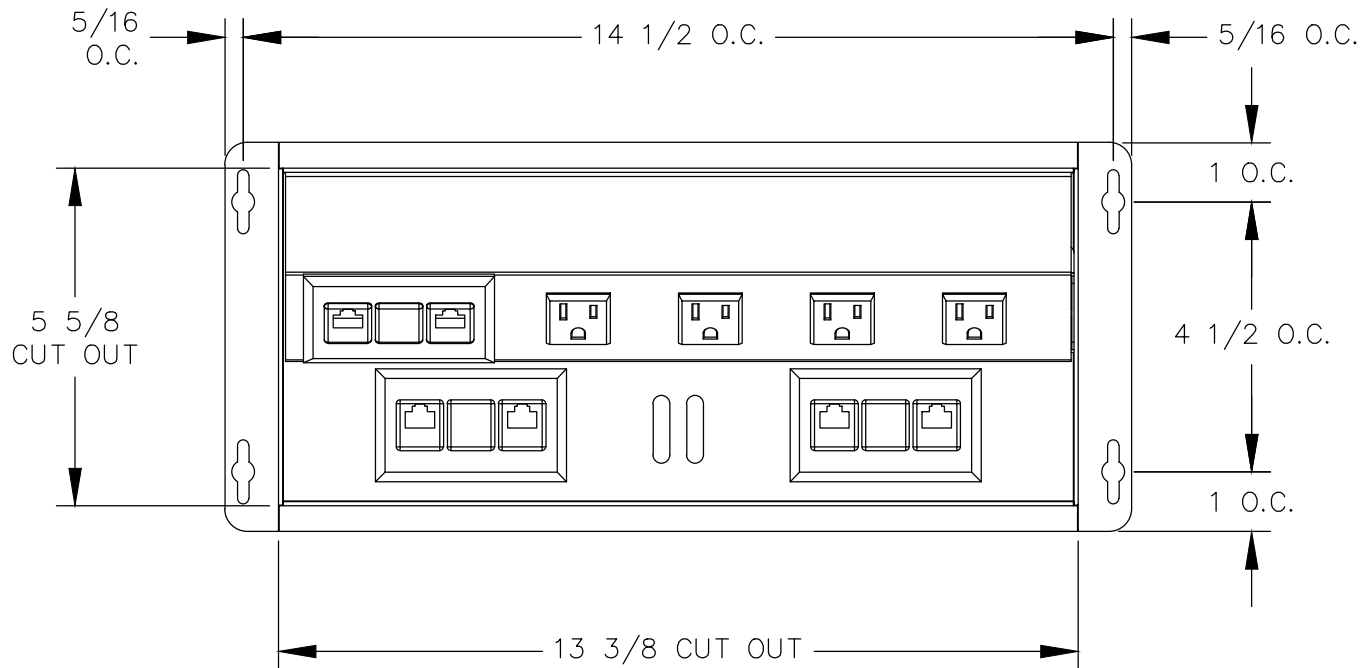
TOP VIEW
