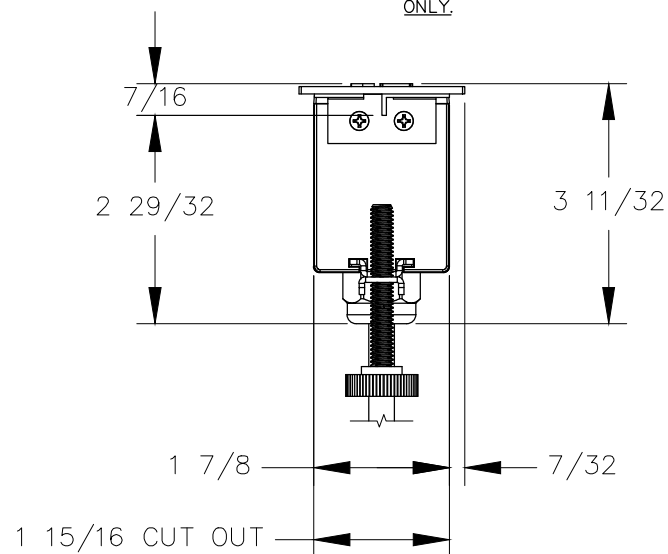
RIGHT VIEW
