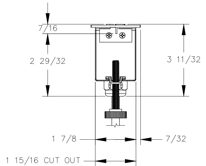
RIGHT VIEW
