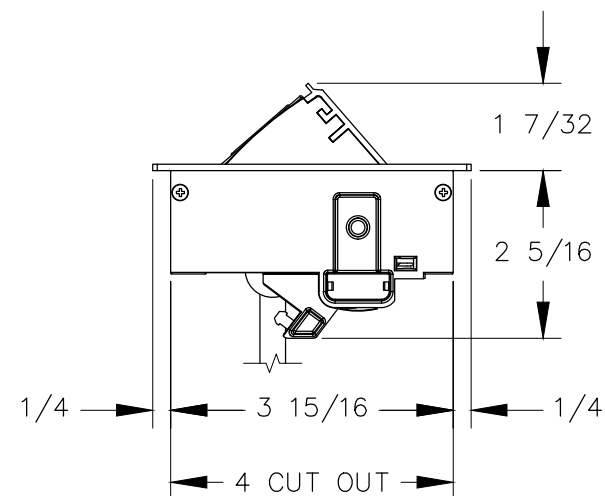
RIGHT VIEW
