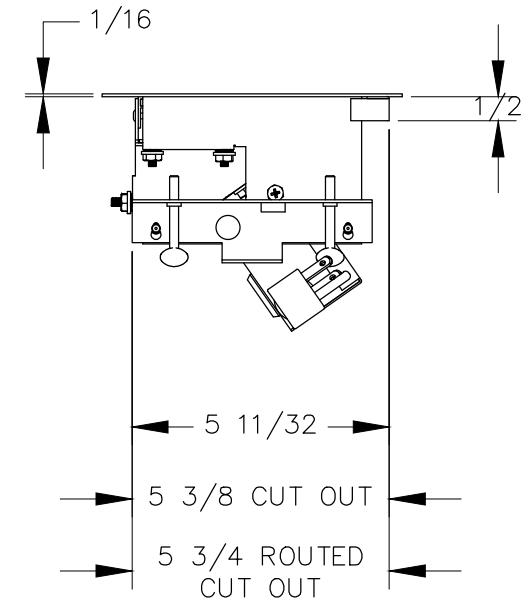
RIGHT VIEW
