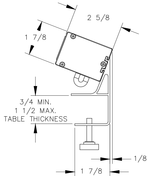
RIGHT VIEW
