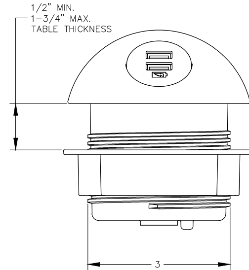
RIGHT VIEW
