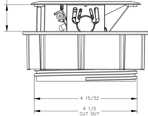
RIGHT VIEW
