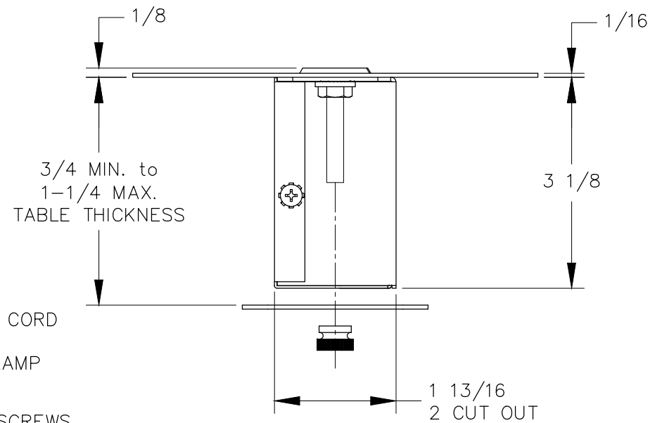
LEFT VIEW
