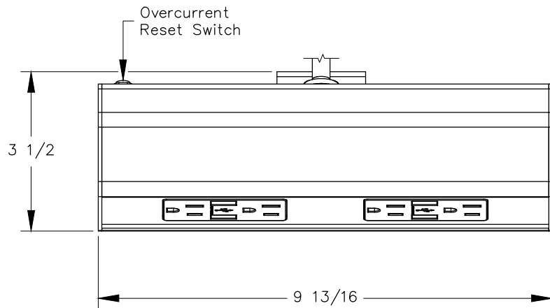
TOP VIEW
