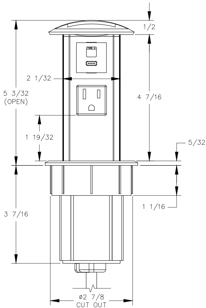
FRONT VIEW
