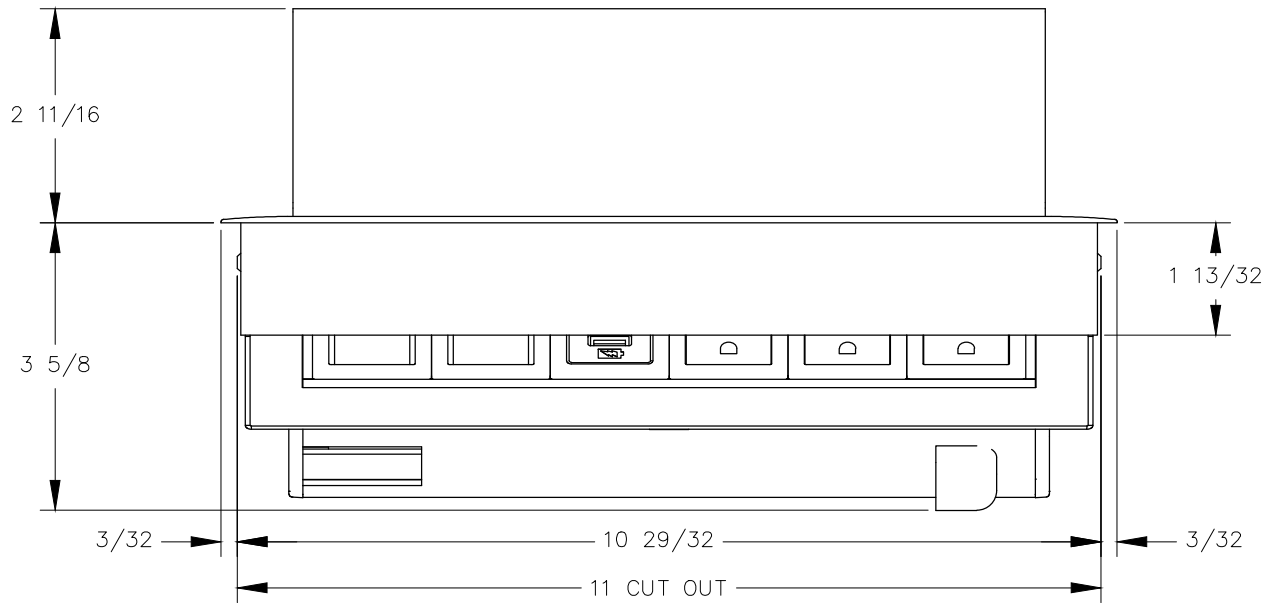
FRONT VIEW
