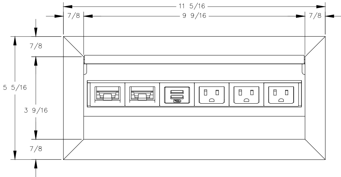
TOP VIEW
