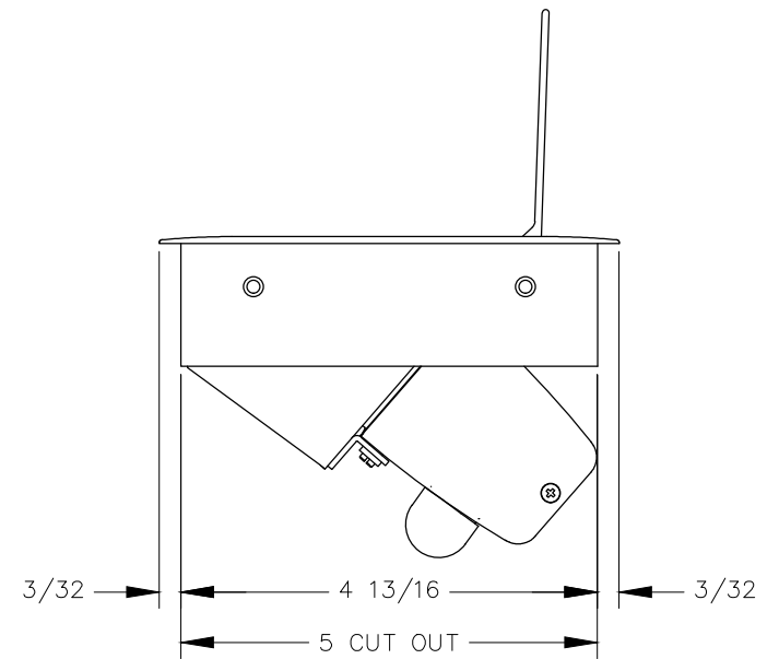
RIGHT VIEW
