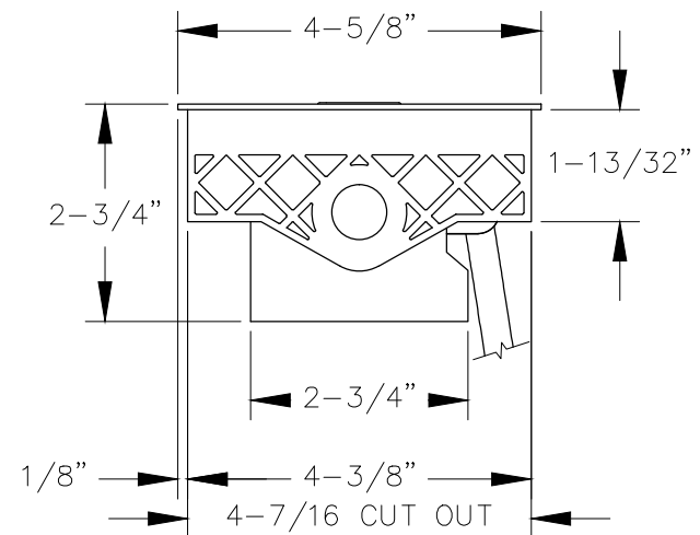
RIGHT VIEW
