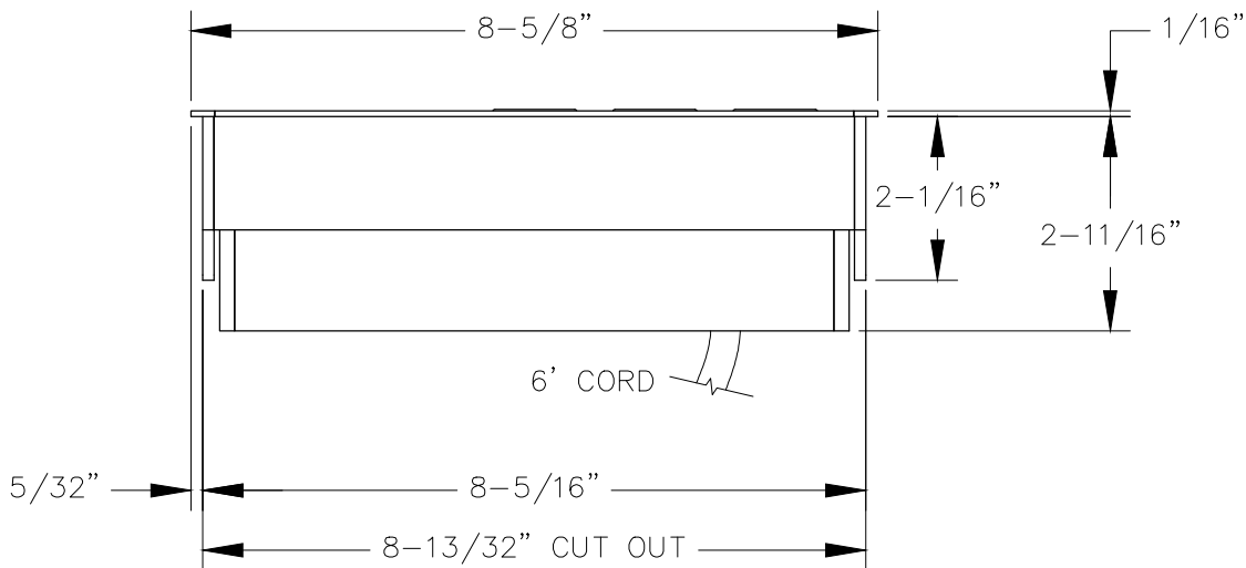
FRONT VIEW
