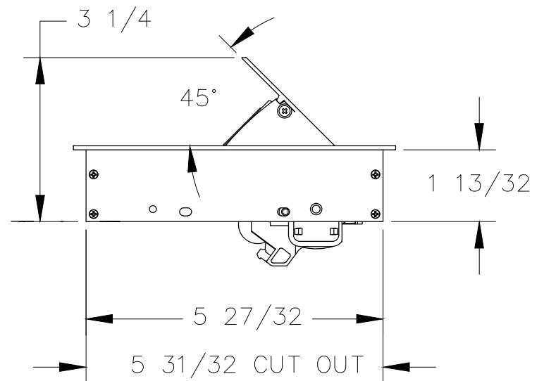
RIGHT VIEW
