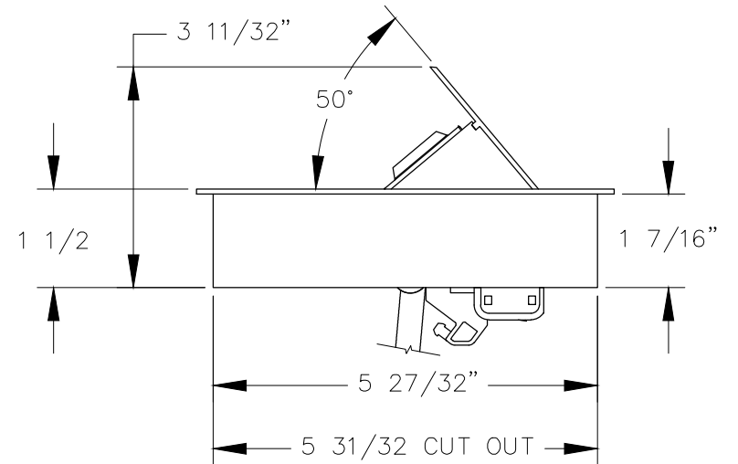
RIGHT VIEW
