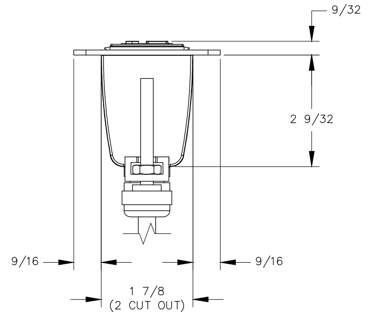
RIGHT VIEW
