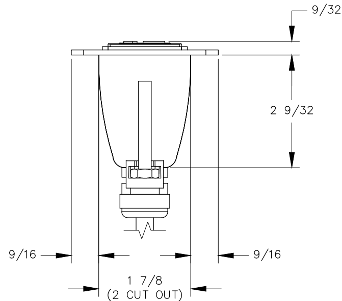
RIGHT VIEW
