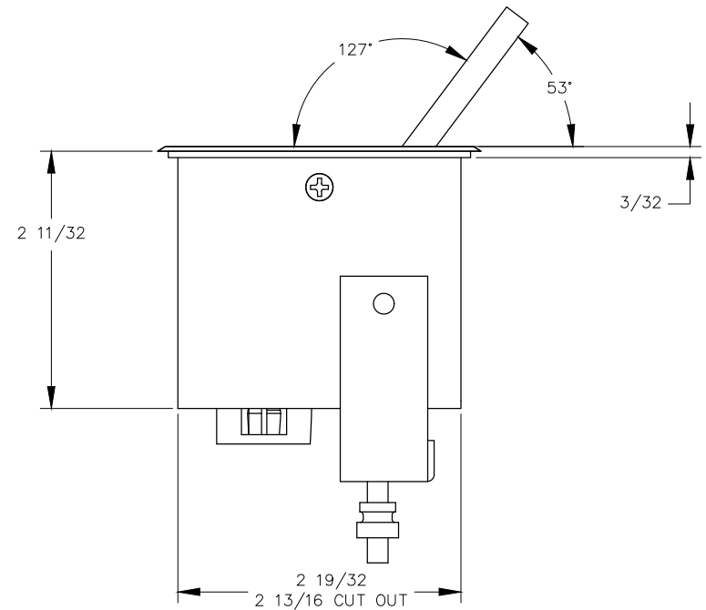
RIGHT VIEW
