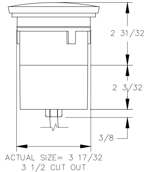
RIGHT VIEW
