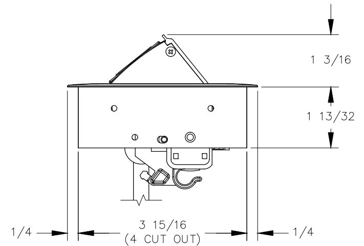
RIGHT VIEW
