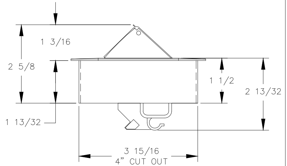
RIGHT VIEW
