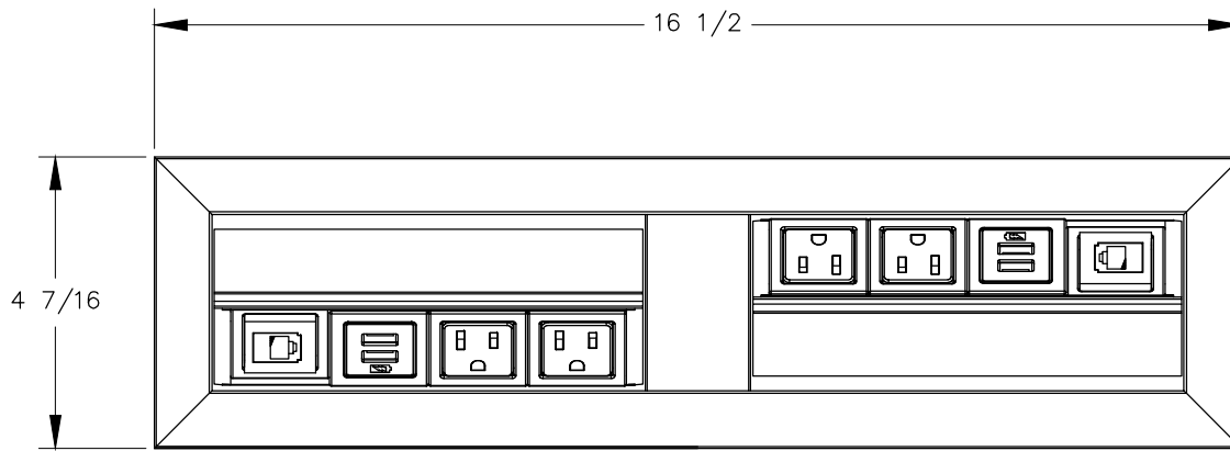
TOP VIEW
