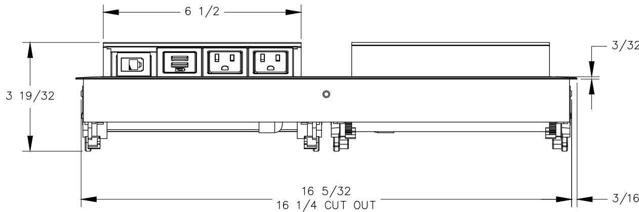
FRONT VIEW
