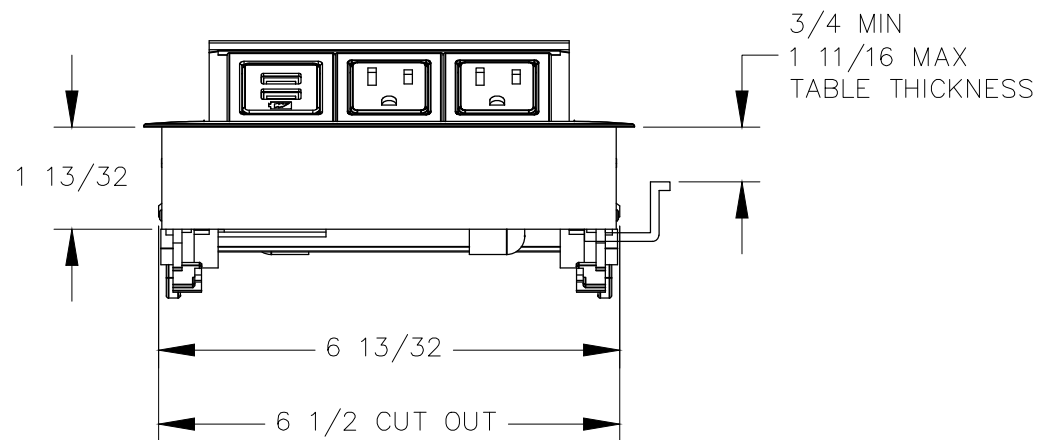
RIGHT VIEW
