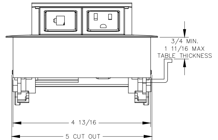
RIGHT VIEW
