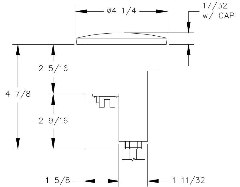
RIGHT VIEW
