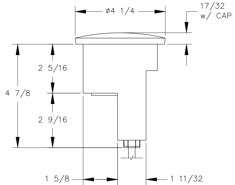
RIGHT VIEW
