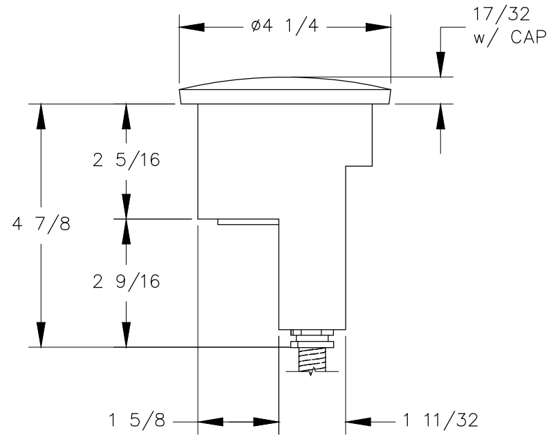
RIGHT VIEW
