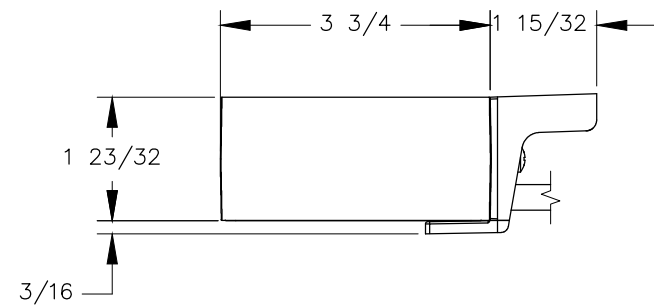
RIGHT VIEW
