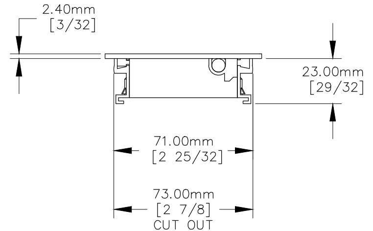
RIGHT VIEW
